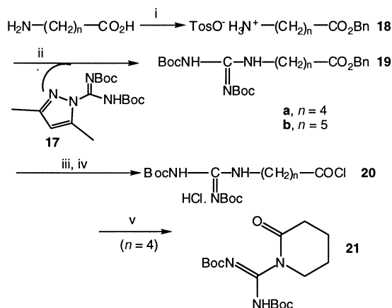
Scheme 2. Synthesis of acid chlorides. Reagents and conditions: (i) PhCH 2 OH, pTos-OH, benzene, reflux, 3 h; (ii) Et 3 N, CH 2 Cl 2 , 20 h, 20 °C; (iii) H 2 , Pd-C, EtOH:EtOAc (1:1), 18 h, 20 °C; (iv) SOCl 2 , CH 2 Cl 2 , 1 h, 30 min, reflux; (v) pyridine, CH 2 Cl 2 , 20 °C.
