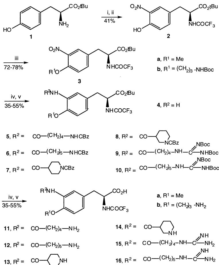
Scheme 1. Synthesis of peptidomimetics (first family). Reagents and conditions: (i) (CF 3 CO) 2 O, 0°C, 2 h; (ii) HNO 3 -HOAc, 10°C, 1 h; (iii) a. CH 3 I, CH 3 CN, K 2 CO 3 , reflux, 48 h; b. BocNH-(CH 2 ) 3 -Br, CH 3 CN, K 2 CO 3 , reflux, 24 h; (iv) H 2 , PtO 2 , EtOH, 4–12 h, 20°C; (v) acid chloride, pyridine, CH 2 Cl 2 , 17 h, 20°C; then column chromatography; (vi) Pd-C, EtOAc, 20°C, 18 h; (vii) CF 3 CO 2 H, 2 h, 20°C.
