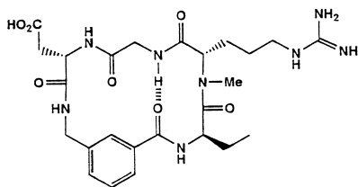
Figure 2. Cyclopeptide DMP728.
