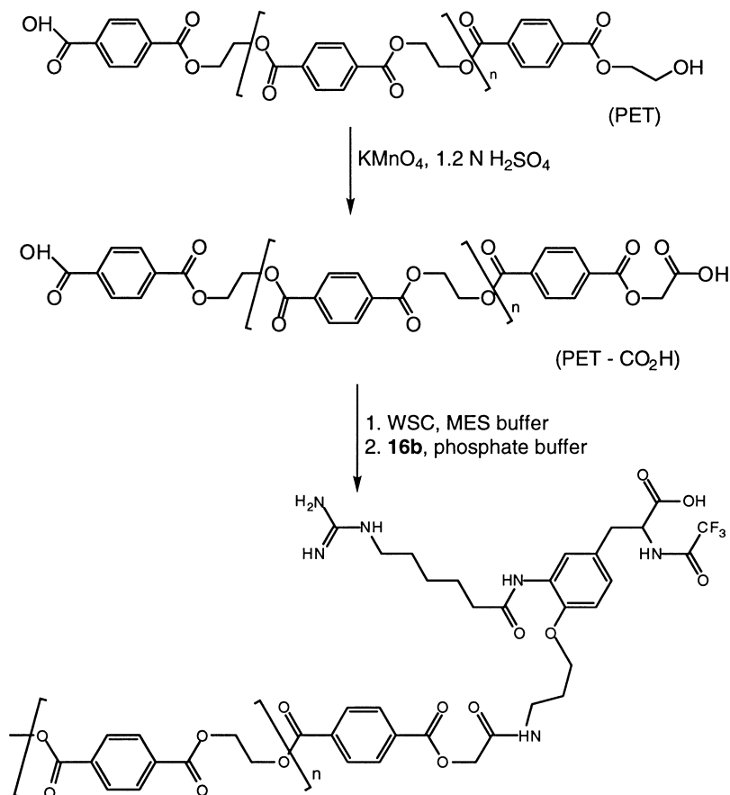
Scheme 4. Covalent coupling of 16a onto the PET membrane surface.
