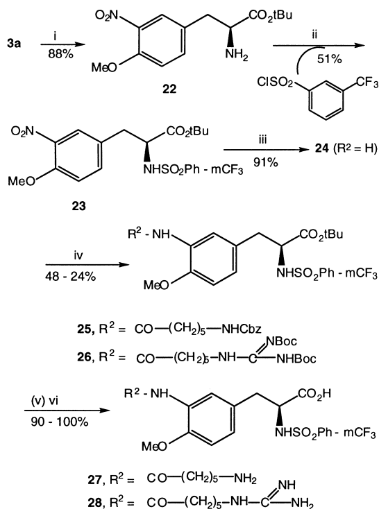
Scheme 3. Synthesis of peptidomimetics (second family). Reagents and conditions: (i) K 2 CO 3 , MeOH:H 2 O (1:1), 17 h, 20 °C; (ii) Et 3 N, CH 2 Cl 2 , 20 h, 20 °C; (iii) H 2 , PtO 2 , MeOH, 17 h 20 °C; (iv) acid chloride, pyridine, CH 2 Cl 2 , 20 h, 20 °C; then column chromatography; (v) H 2 , Pd-C, EtOH:EtOAc (1:1), 18 h, 20 °C; (vi) CF 3 CO 2 H, 2 h 30 min, 20 °C.
