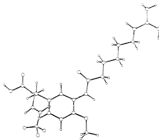
Figure 3. Cyclopeptide c(RGDFV).
