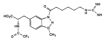
Figure 4. Peptidomimetic 16a .
