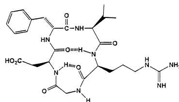
Figure 3. Cyclopeptide c(RGDFV).
